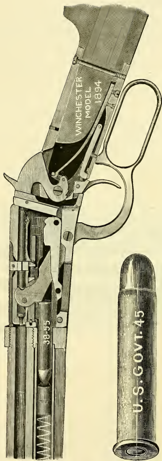
The Winchester (1894) Rifle and .45 Cartridge.
